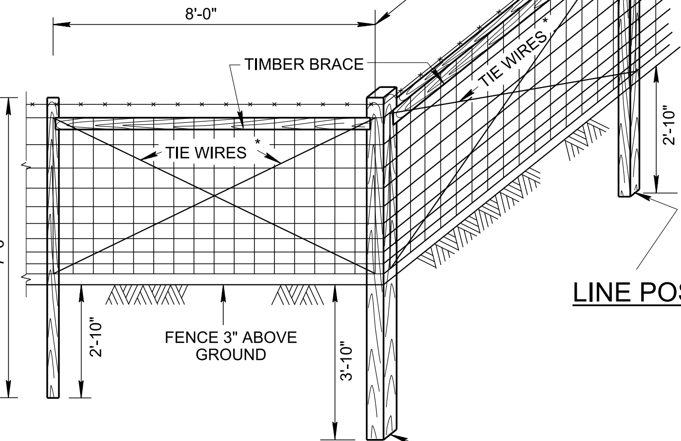
CORNER POST ITEM NO. 707-03.02
