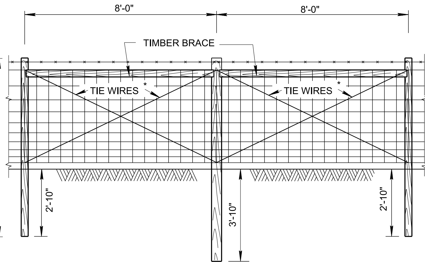
BRACED LINE POST ITEM NO. 707-03.02
