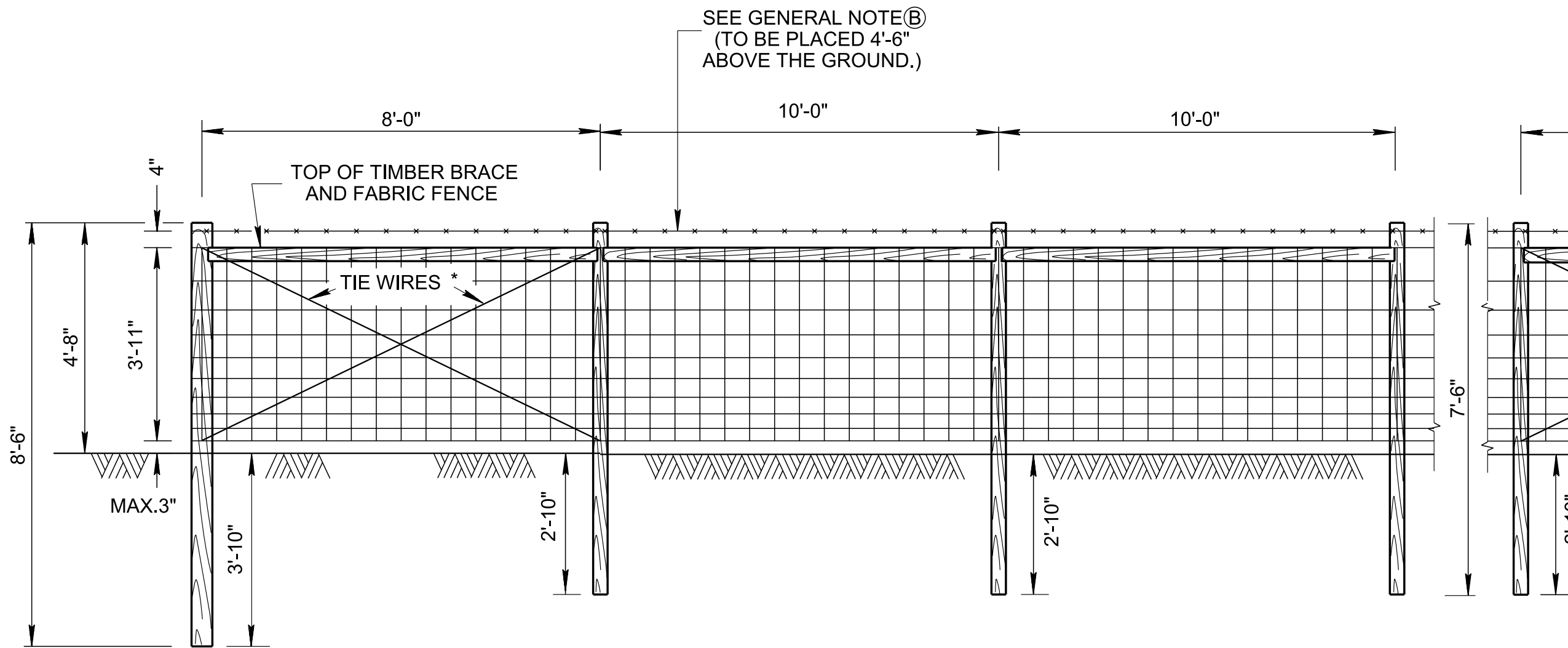
LINE POST
